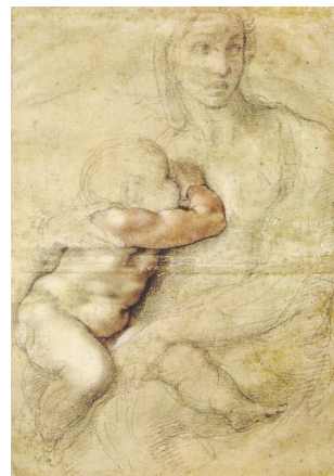
M 11
